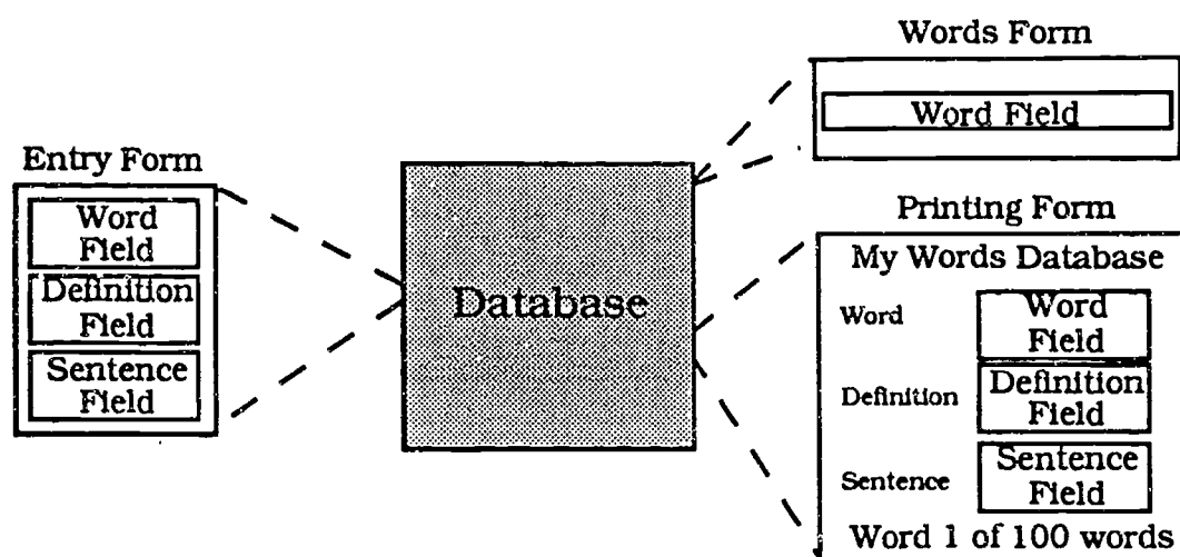
Figure 4 — Different forms for a database.
